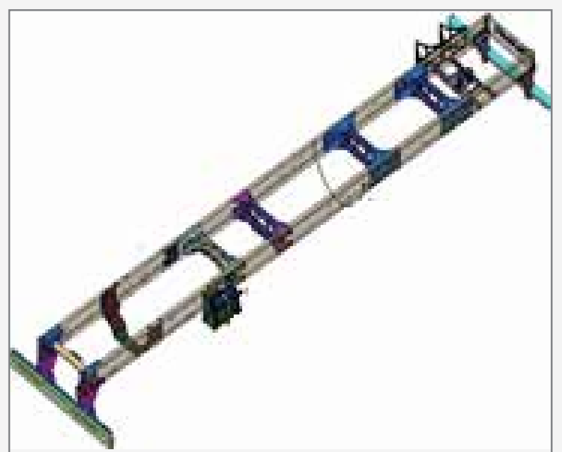
High Strength Low Alloy Chassis for Higher Strength and a Greater Sense of Security
