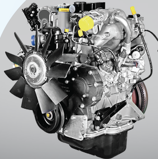
Automatic Belt Tensioner No manual belt tensioning required
